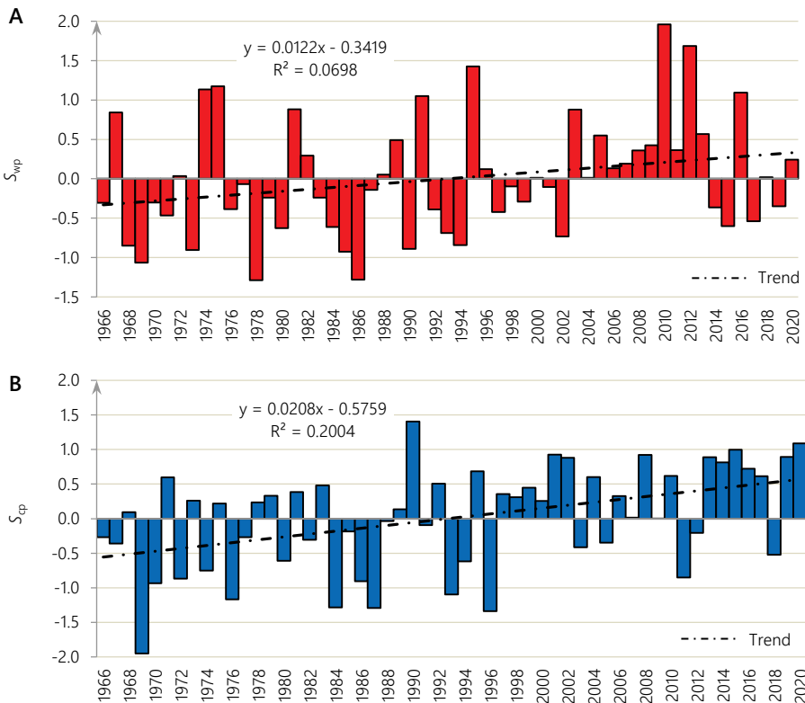
Figure 6. Long-term dynamics of the Pedy index for warm— S_{wp} (A) and cold— S_{cp} (B) periods.
