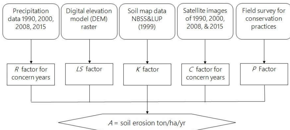
Figure 2. RUSLE methodology flow chart.
