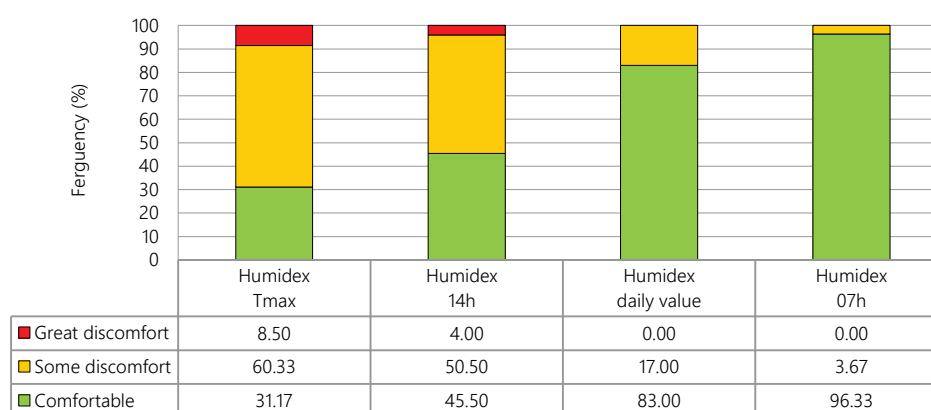
Figure 1. Frequency of the Humidex heat stress categories during June (1998–2017) in Niš.
