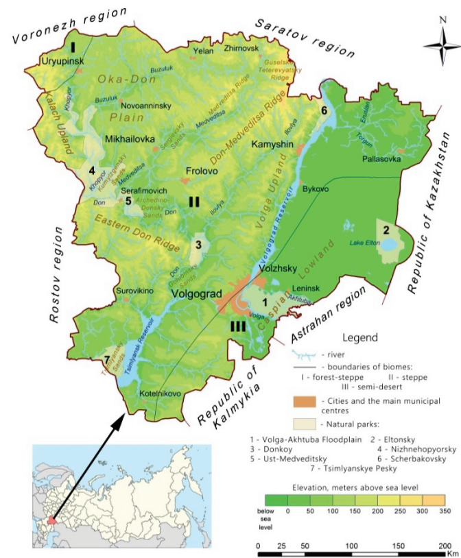
Figure 2. Physical map of the Volgograd region.
